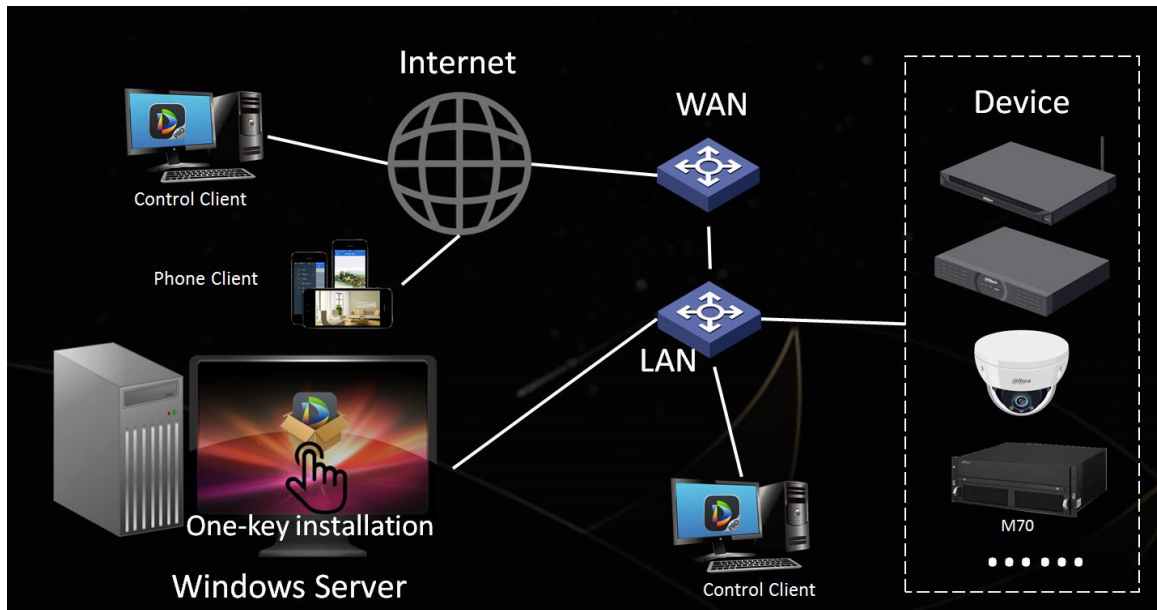
Figure 1-1 DSS Pro networking
