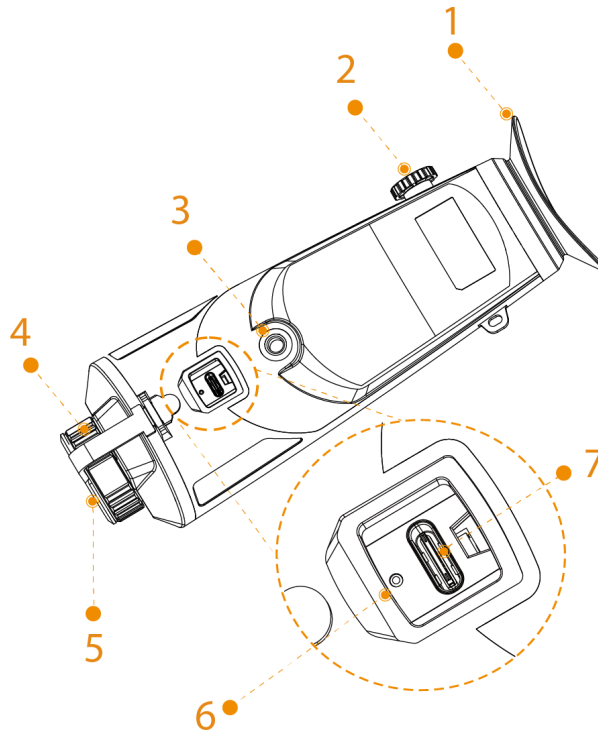
Figure 2-3 Port description (25 mm&35 mm)
